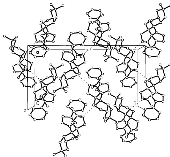
Figure 4. The arrangement of the molecules in the unit cell.
