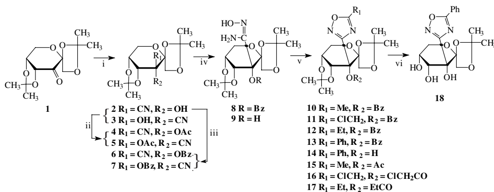
Scheme 1. Reagents and conditions: (i) NaCN, TBAB, rt, \text{CH}_2\text{Cl}_2\text{--H}_2\text{O} ; (ii) \text{Ac}_2\text{O}\text{--Py} , rt; (iii) \text{BzCl}\text{--Py} , 0^\circ\text{C}\text{--rt} ; (iv) \text{NH}_2\text{OH}\text{--CH}_3\text{OH} , reflux; (v) \text{Ac}_2\text{O} , \text{ClCH}_2\text{COCl} , (\text{CH}_3\text{CH}_2\text{CO})_2\text{O} or benzoyl chloride, \text{N}_2 , 80 or 120\text{--}130^\circ\text{C} ; (vi) \text{CF}_3\text{CO}_2\text{H} (90%)– \text{CH}_2\text{Cl}_2 , reflux, 24h, 80%.
